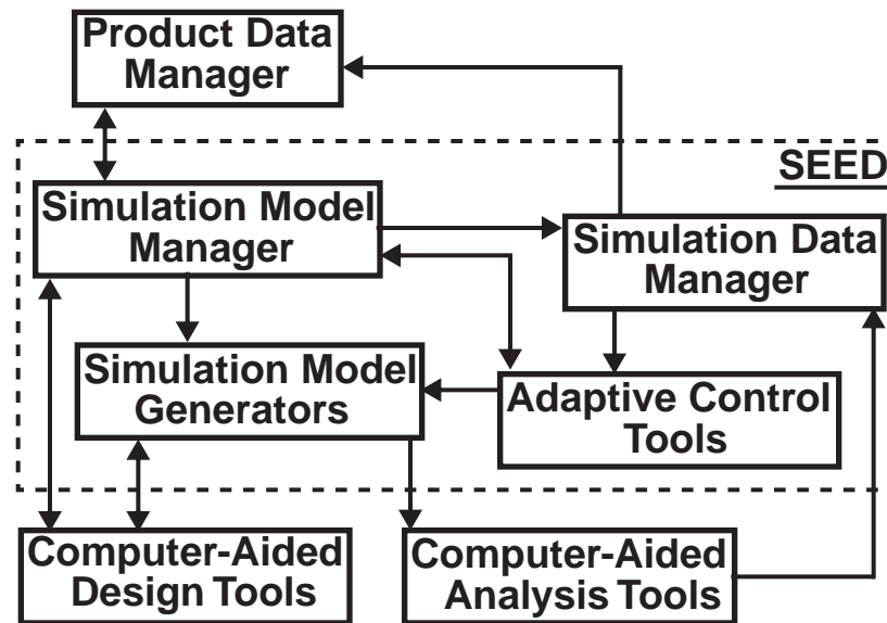
Figure 1. Functional components needed for simulation-based design with the four new components in the dashed box defining the Simulation Environment for Engineering Design (SEED).
