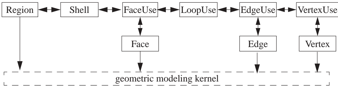
Figure 4. Model topological adjacency information and relation to model geometry.
