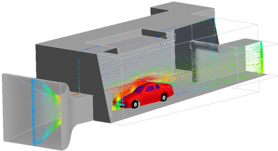
Figure 11. Overall wind tunnel flow results.
