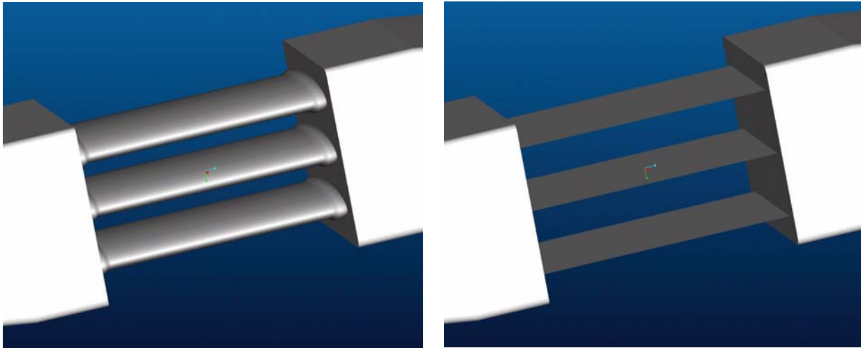
Figure 7. Dimensional reduction for heat exchanger.
