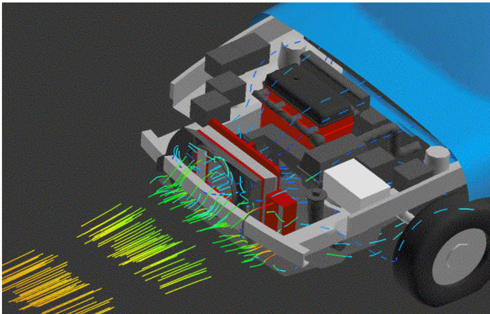
Figure 12. Flow results in the critical under the hood region.
