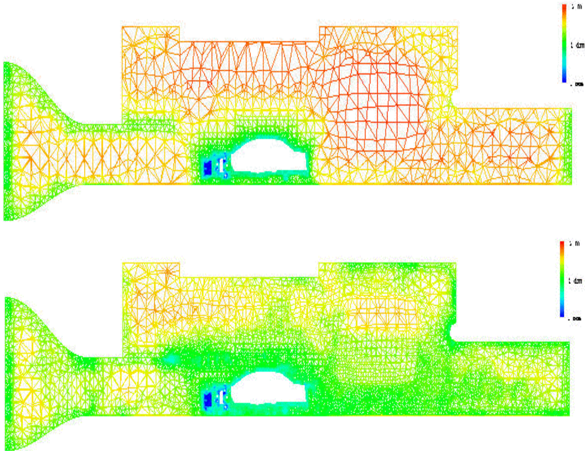
Figure 13. Initial and adaptively refined mesh.
